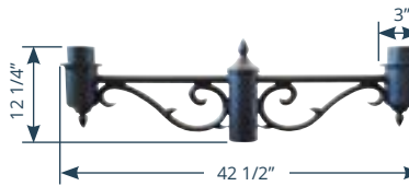
P7327 Post Mount Double Lighting Arm - Made of extruded and cast aluminum - Decorative Scrolls
